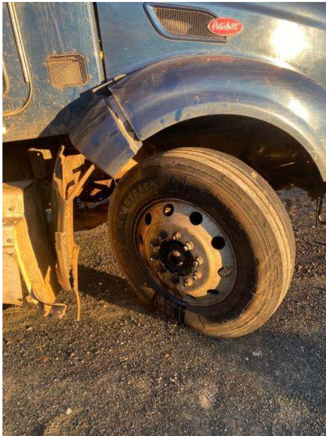
Right front wheel/suspension damage
